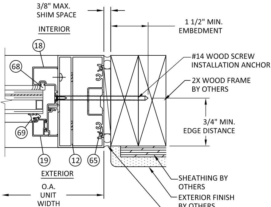
L 5 HORIZONTAL SECTION TRANSOM JAMB - 2X WOOD FRAME
