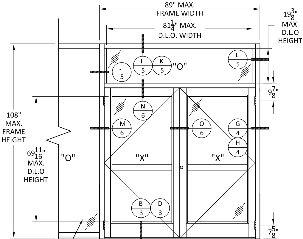
ELEVATION B DOUBLE DOOR WITH TRANSOM AND SIDELITE
