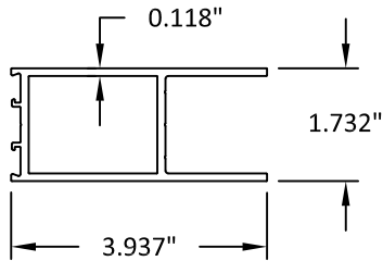
TOP RAIL
