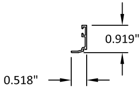
EXT. GLASS STOP (1")
