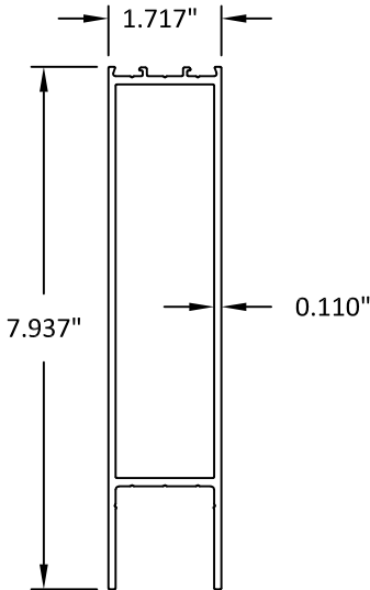
8" BOTTOM RAIL
