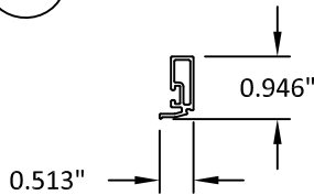
INT. GLASS STOP (9/16")
