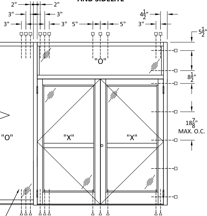
ANCHOR LAYOUT B DOUBLE DOOR WITH TRANSOM AND SIDELITE
