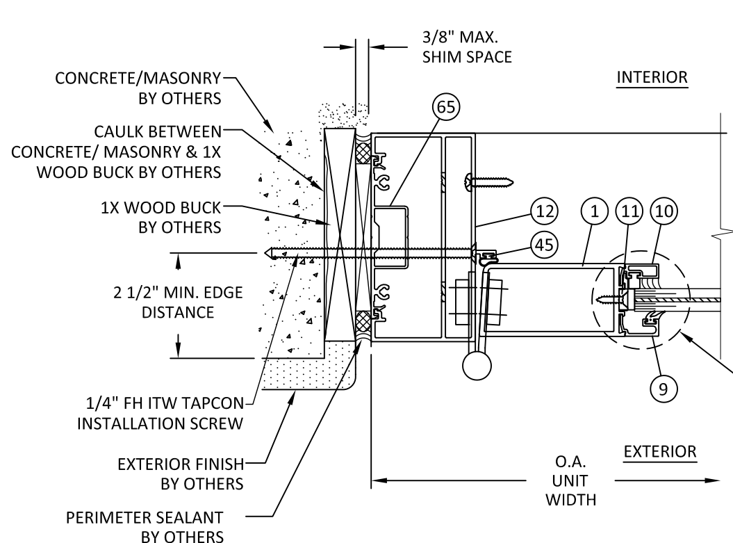
E HORIZONTAL SECTION 4 DOOR JAMB - CONCRETE/MASONRY STANDARD BUTT HINGE
