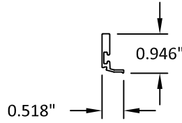
INT. GLASS STOP (1")
