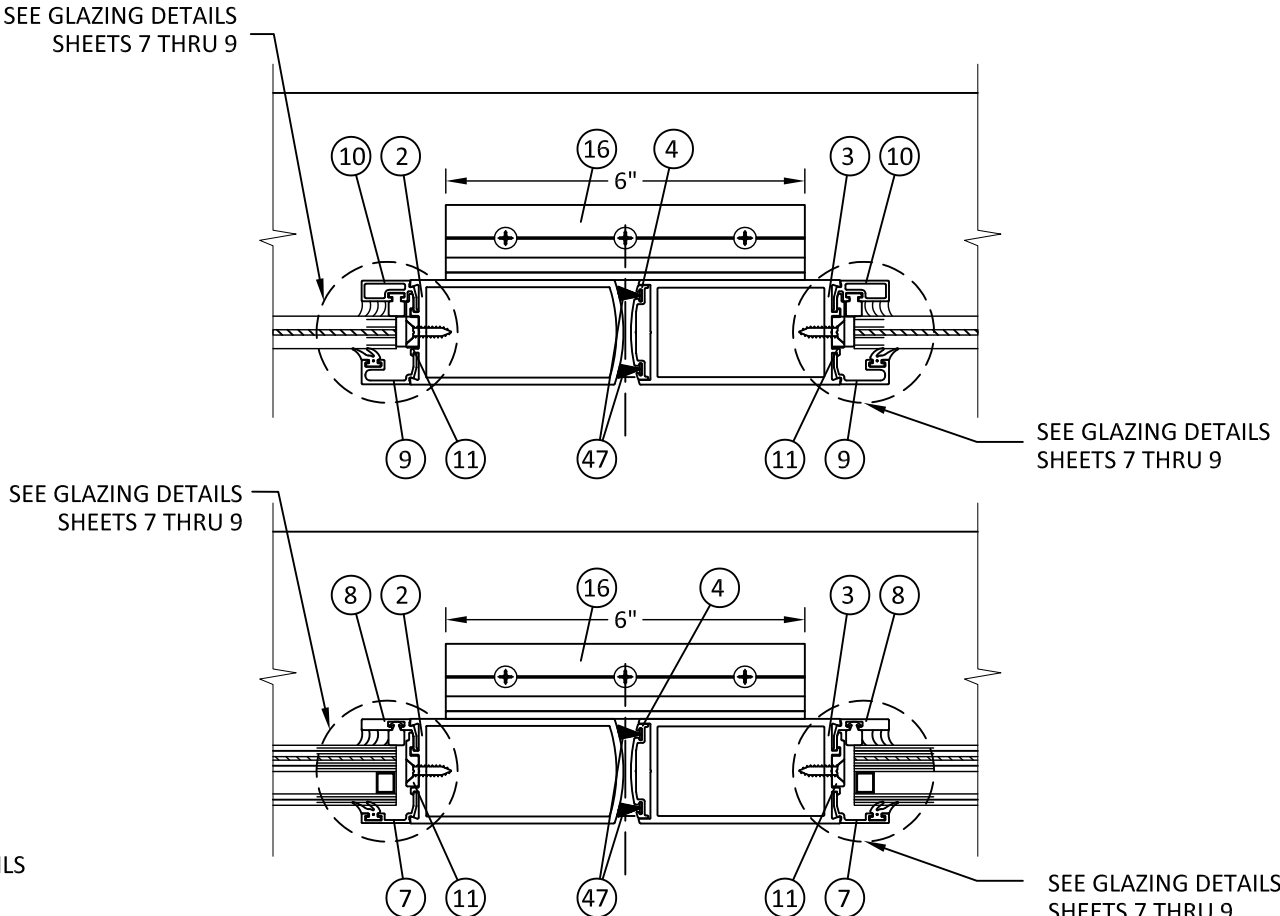
O 6 HORIZONTAL SECTION MEETING STILE
