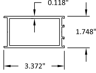
MEETING STILE (ACTIVE)
