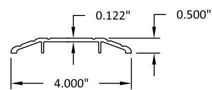
15 4" THRESHOLD
