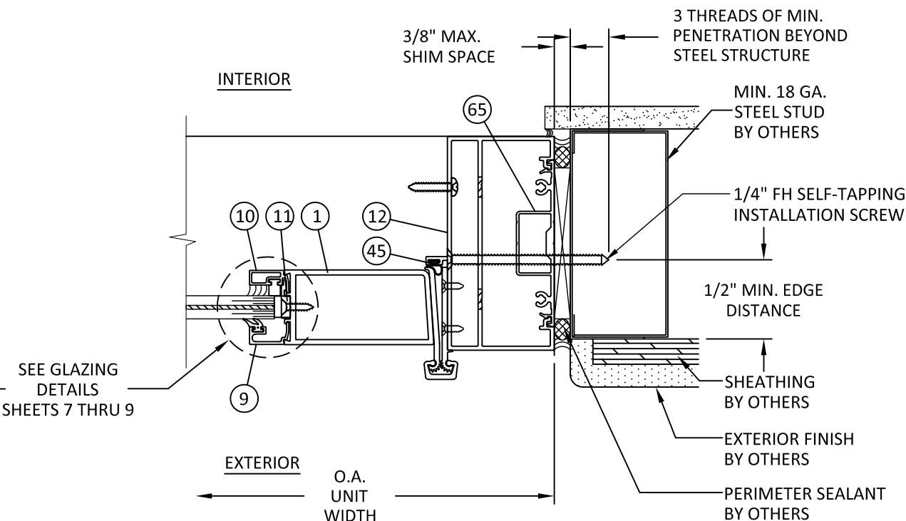
G HORIZONTAL SECTION 4 DOOR JAMB - STEEL STUD ROTON CONTINUOUS HINGE
