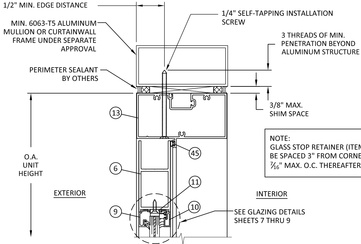
A 3 VERTICAL SECTION DOOR HEAD - ALUMINUM MULLION
