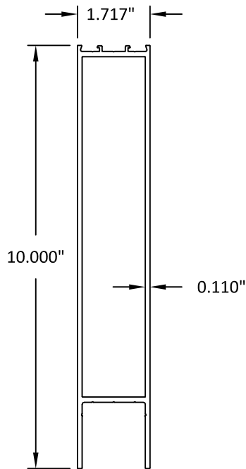
10" BOTTOM RAIL
