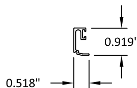
EXT. GLASS STOP (9/16")
