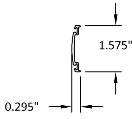
EXT. GLASS STOP (9/16")
