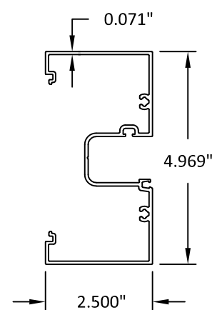
51 HEAD/JAMB/MULLION (MONO)
