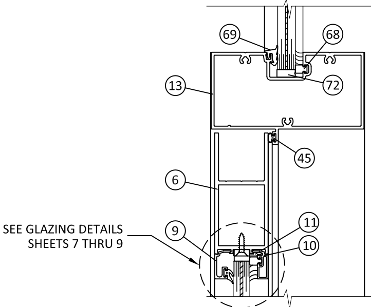
N 6 VERTICAL SECTION TRANSOM BAR
