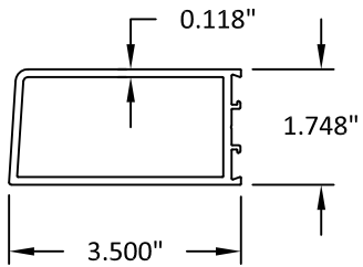
TOP RAIL
