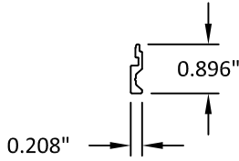
10" BOTTOM RAIL
